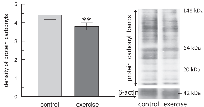
Fig. 2. Protein carbonyl content in the hippocampus decreased by long-term exercise compared to the sedentary control group (** p < 0.01 vs. control). Columns represent means \pm SEMs for six animals per group. The representative Western blots show the immunoreactivities of protein carbonyls and \beta -actin (used as a loading control) at the right side of figure.
