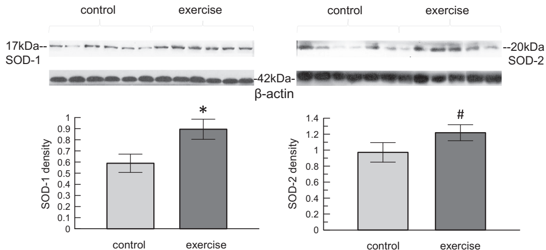
Fig. 3. Intracellular SOD-1 protein levels (left side) and mitochondrial SOD-2 protein content (right side) are shown in the hippocampus of 15-month-old aging female rats. SOD-1 protein levels are increased as a result of exercise (* p < 0.05 vs. control). The right side histogram represents that SOD-2 protein levels tended to be increased in exercised rats compared to the sedentary control group (# p = 0.087 vs. control). Columns represent means \pm SEMs, n = 6 . The representative western blots taken from each individual rats show the immunoreactivities of SOD-1 and SOD-2 (upper lines) and below that of \beta -actin (used as a loading control).
